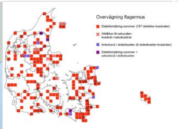
Fig. 2. Based on knowledge about bat species occurrence in each of the square in Fig.1. 157 squares of special interest were selected (red squares). In these squares sites, and some-times satellite sites, were selected for surveillance for bat species richness. Red rasters: satellite sites in neighbouring squares. Blue rasters: surveillance in well know winter roosts.
