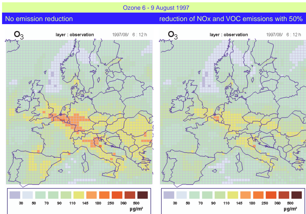
Figure 1. Visualisation of ozone concentrations over Europe on August 6 at 12h: without emission reductions (left) and with 50% reduction of NO x and VOC emissions (right)
